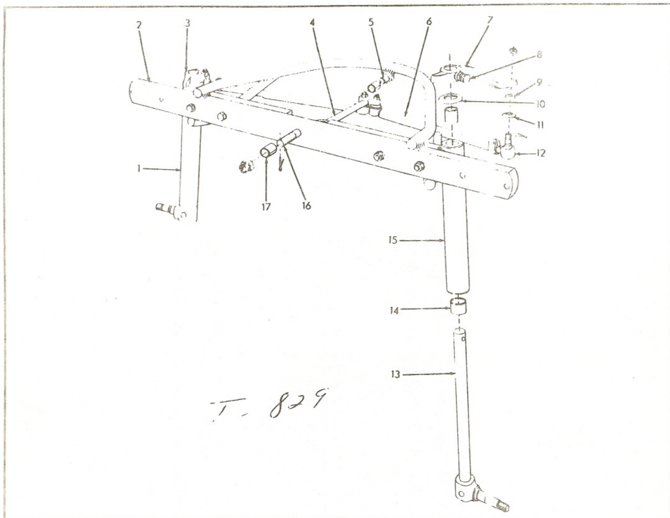
FRONT AXLE
