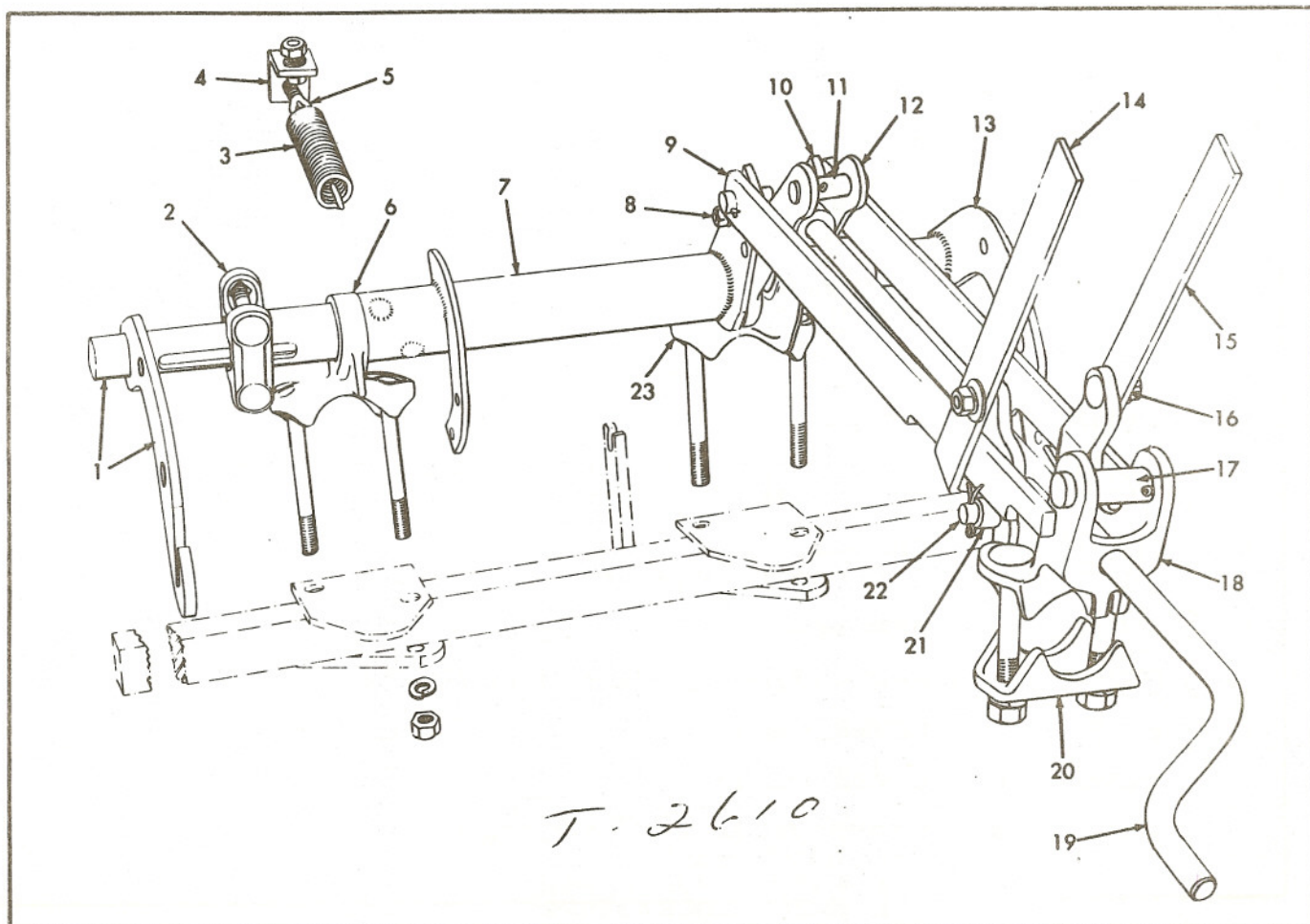
HYDRAULIC LIFT SHAFT Split Type
