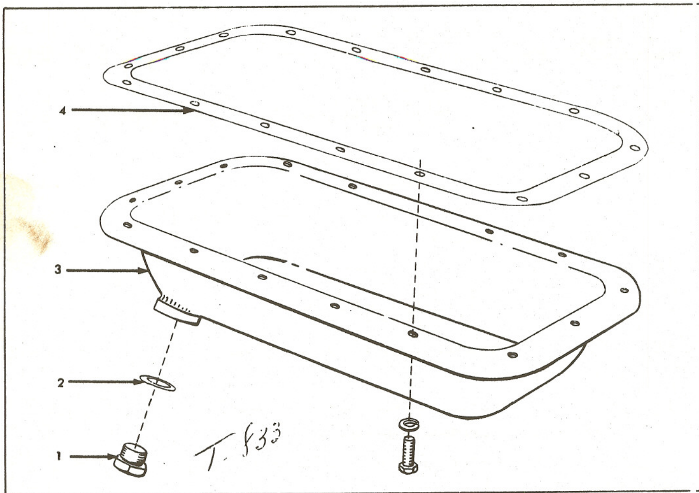
OIL SUMP
