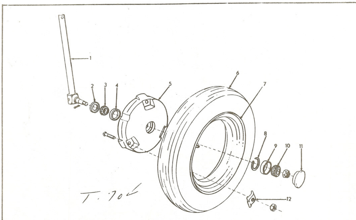
FRONT WHEEL
