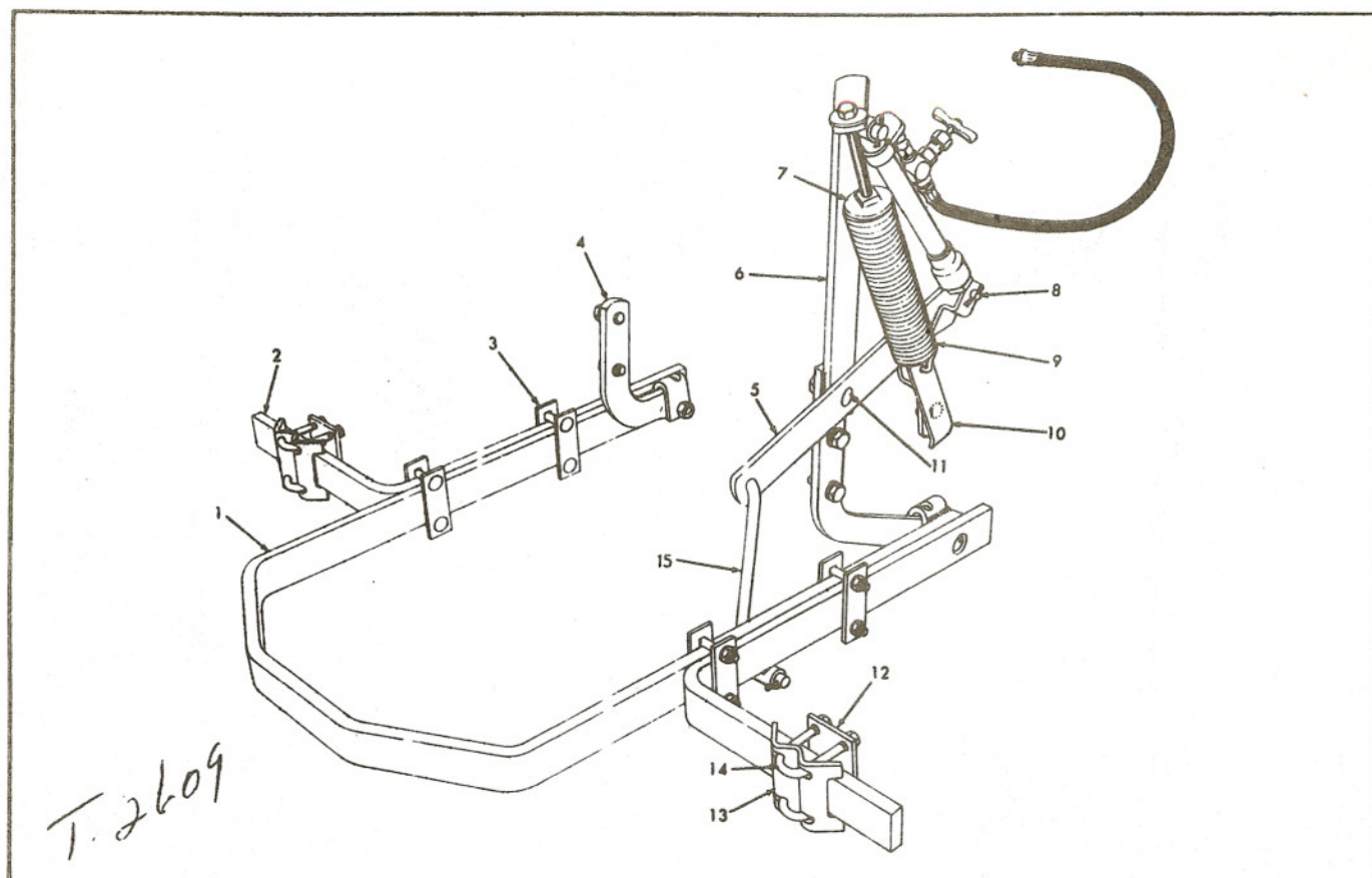
REAR FURROWING BAR WITH HYDRAULIC LIFT
