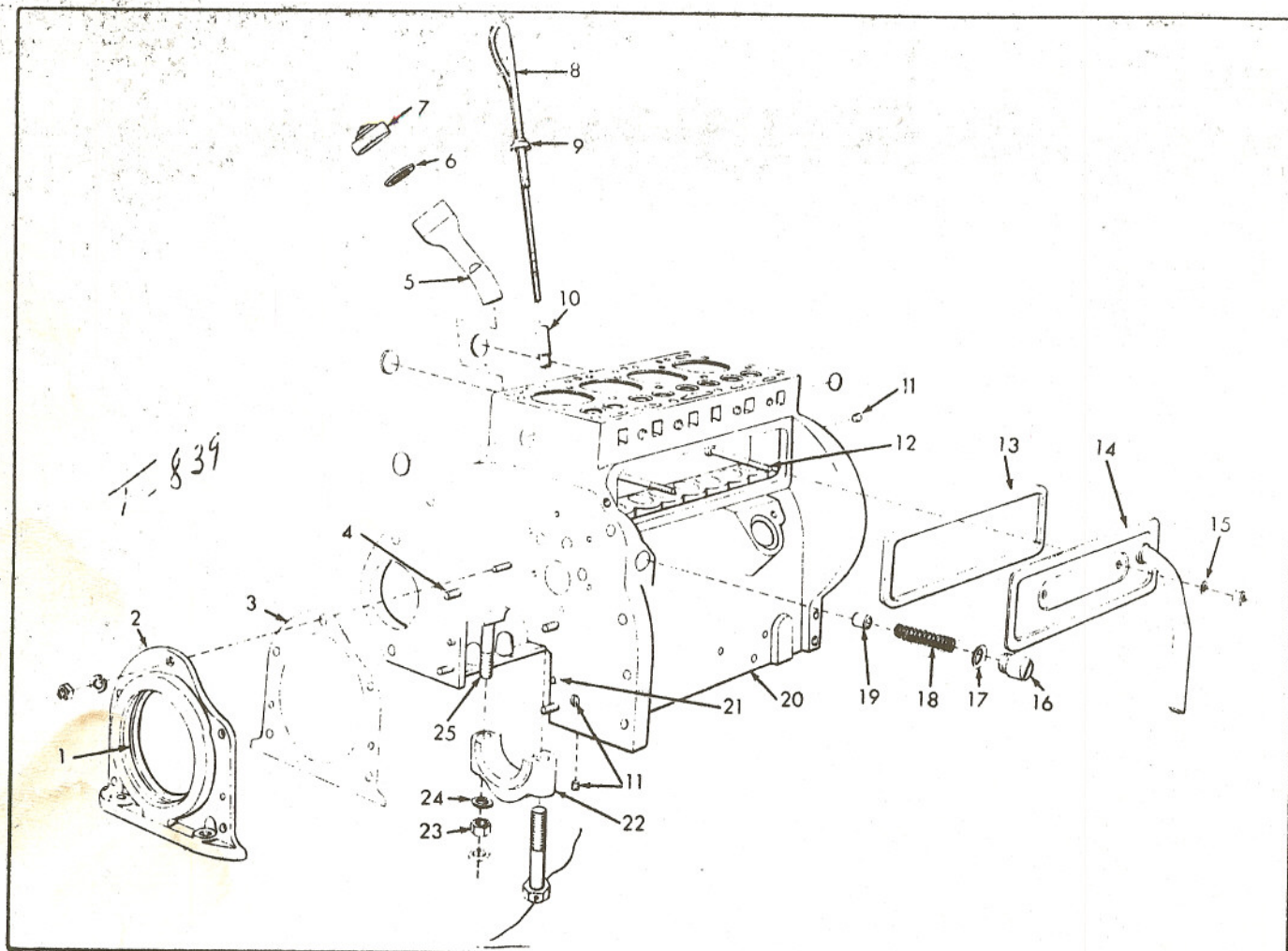
CYLINDER BLOCK
