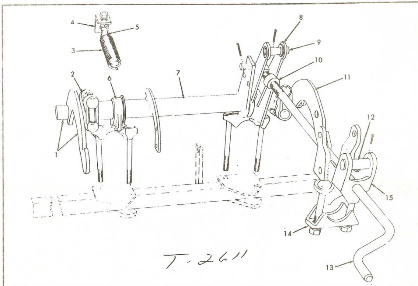
HYDRAULIC LIFT SHAFT Solid Type
