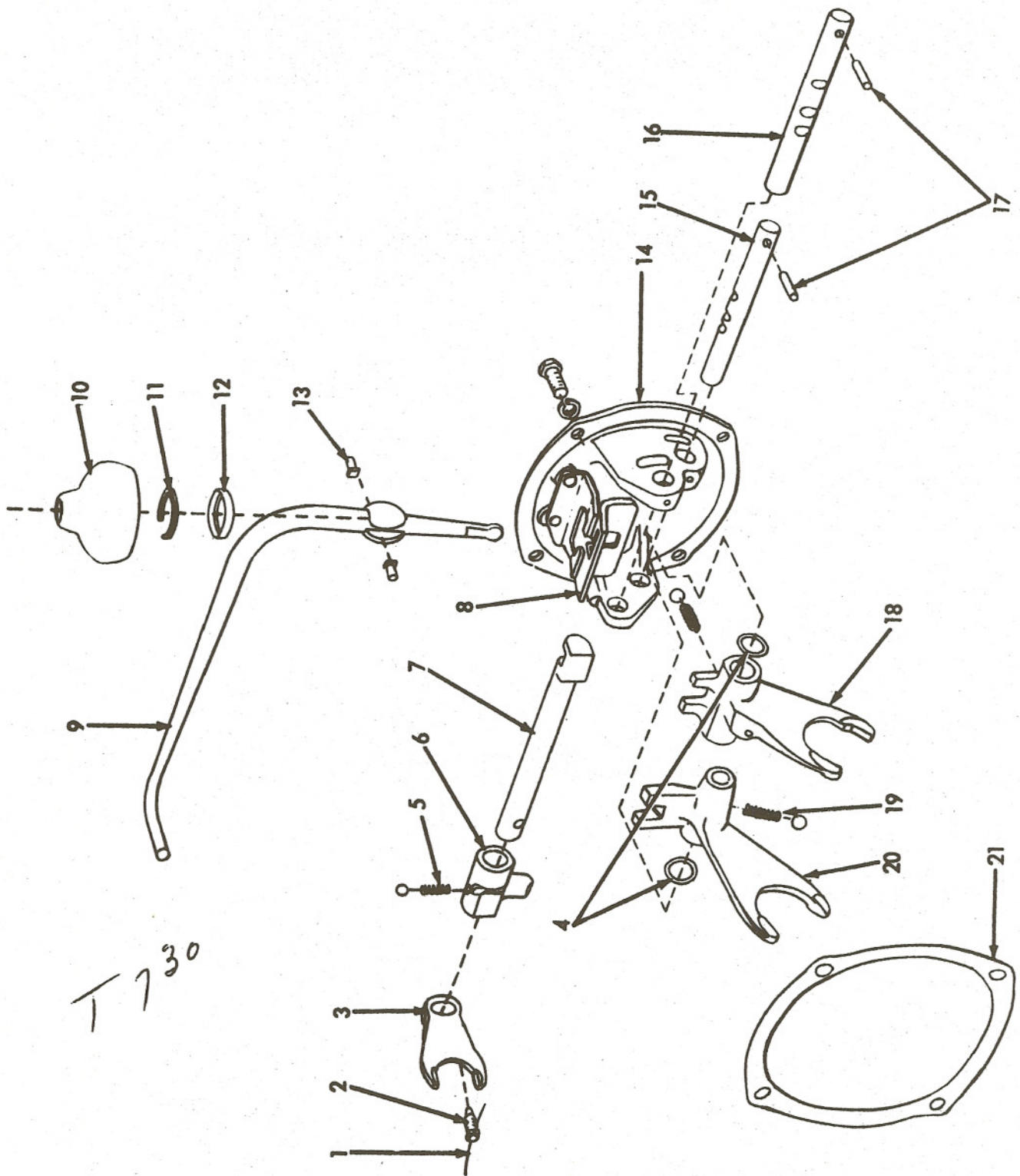
TRANSMISSION CONTROL
