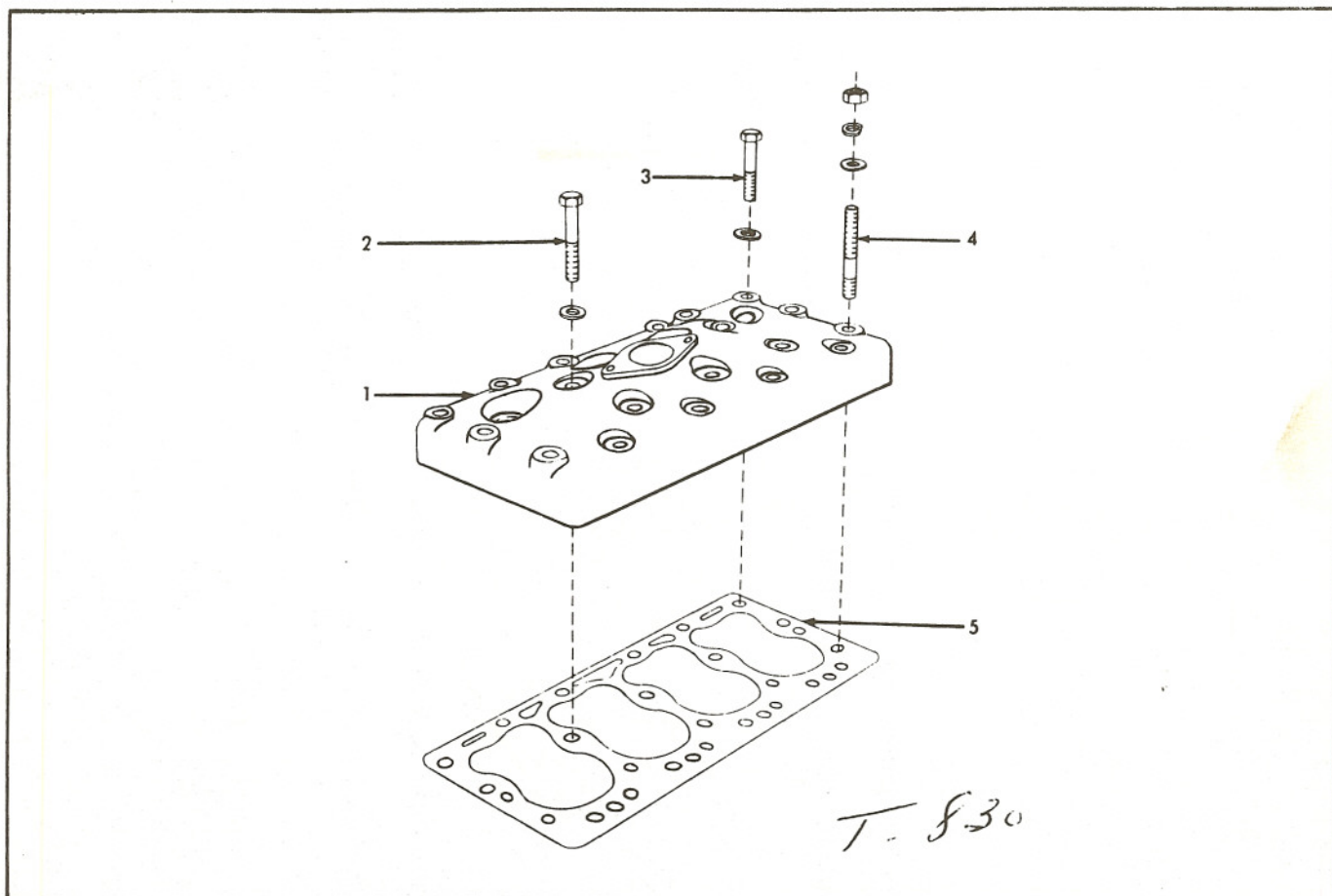
CYLINDER HEAD
