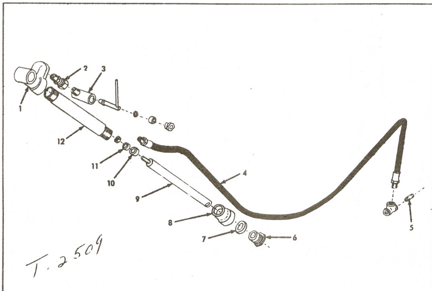
REAR HYDRAULIC RAM
