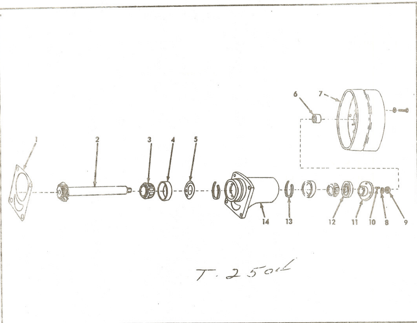
BELT PULLEY Used with Hydraulic Pump
