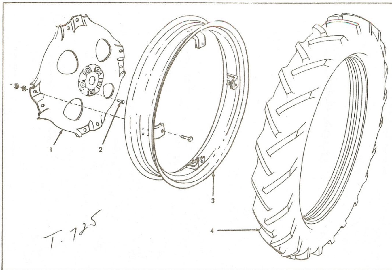
REAR WHEEL
