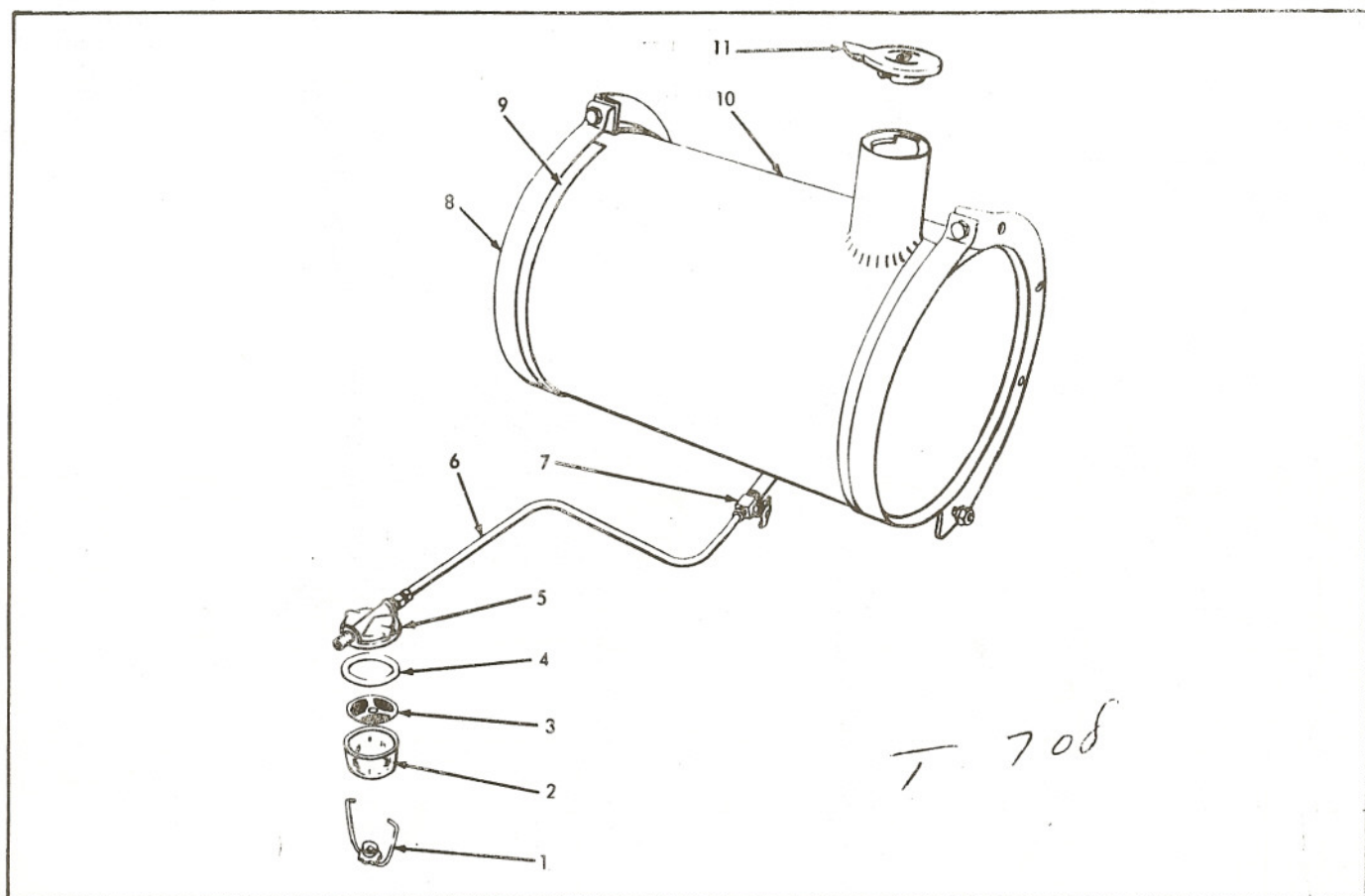
FUEL TANK, FILTER & LINES
