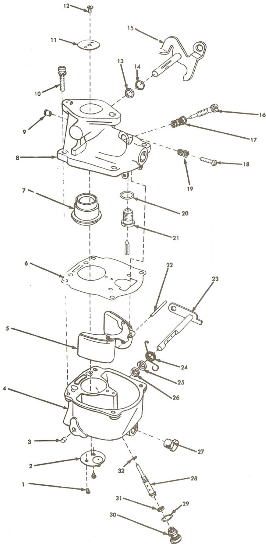
CARBURETOR
