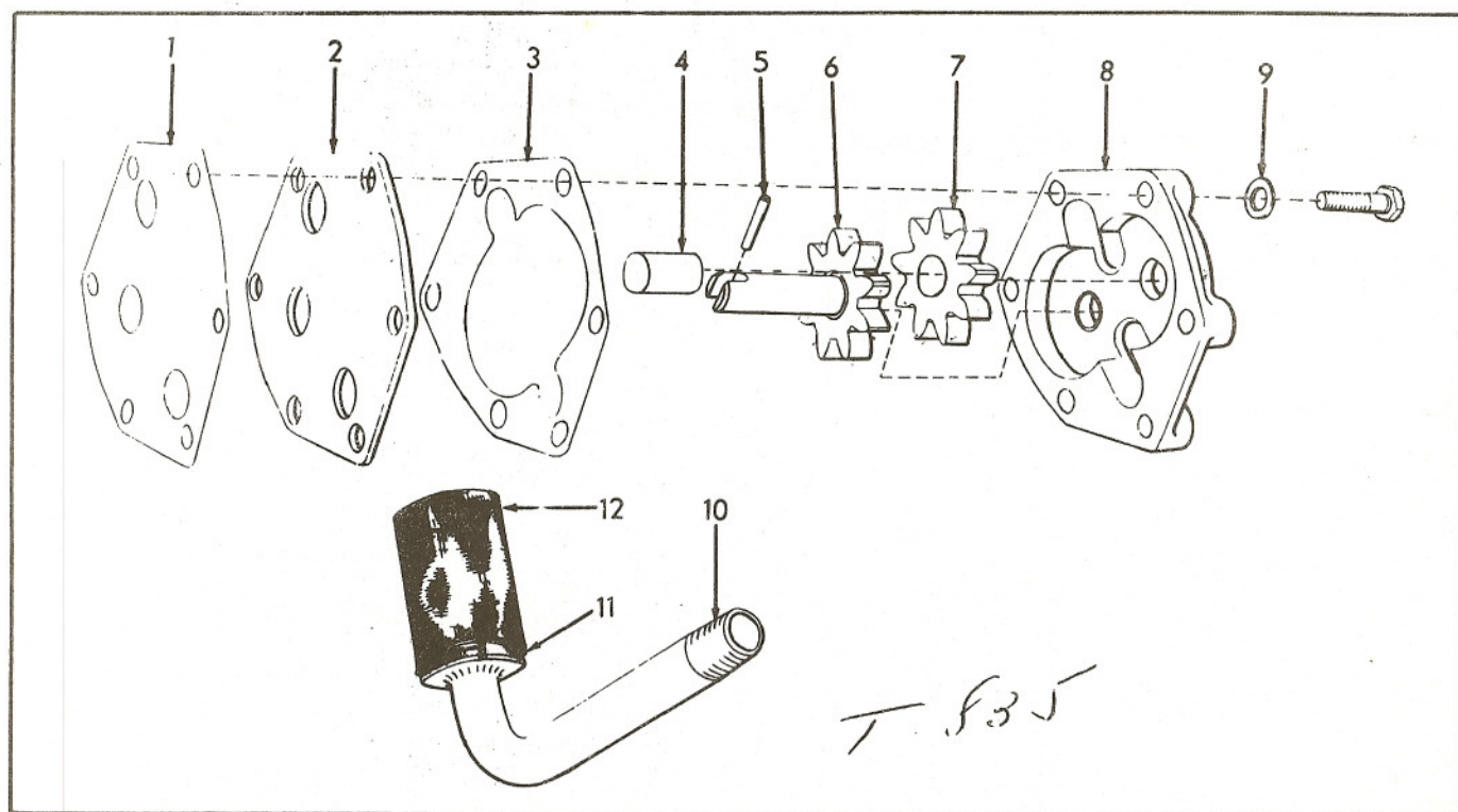
OIL PUMP
