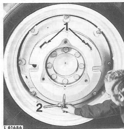
1 Crochets
